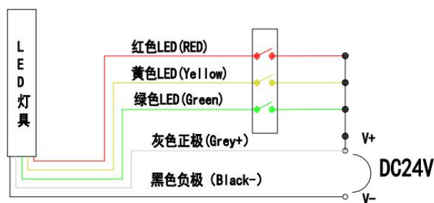
DC24V共负 (Common -)
